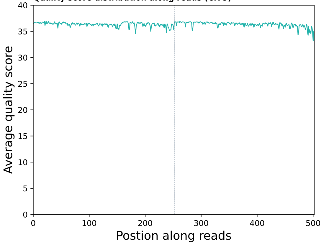
Quality score distribution along reads (CK-3)
